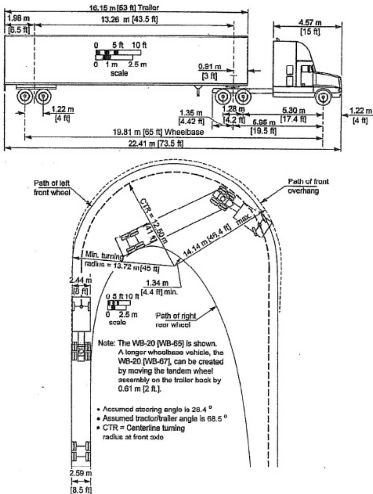
Figure 14: Minimum Turning Path for Interstate Semitrailer (WB-20 [WB-65 and WB-67]) Design Vehicle
