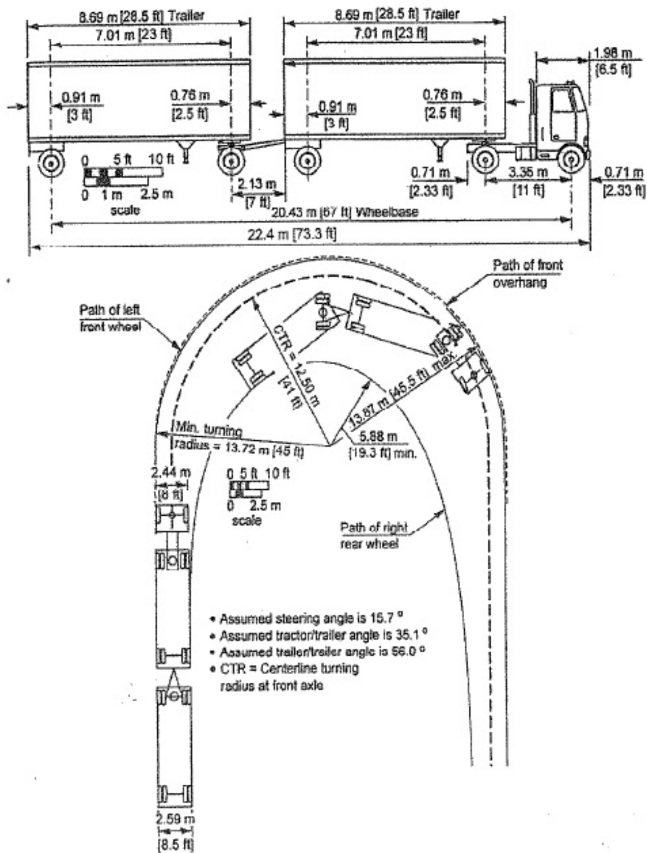
Figure 15: Minimum Turning Path for Double-Trailer Combination (WB-20D [WB-67D]) Design Vehicle
